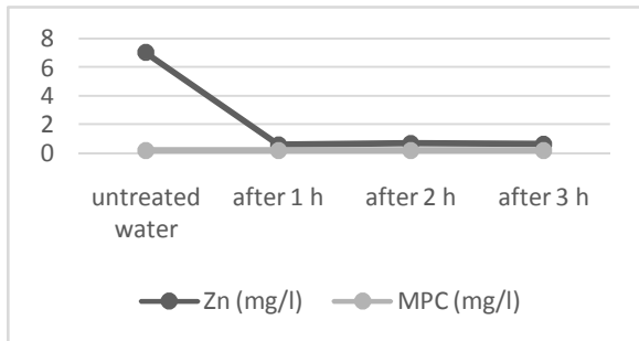
Fig. 3 Content of Zn in mine water after treating with CaCO 3
