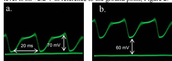
Figure 2. Waveform of the signal on the ends of the indicator a) When in null position of the arrow b) When in drift of the arrow
