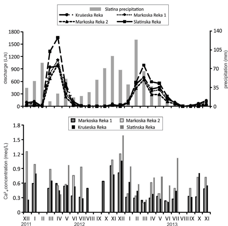
Fig. 6. \text{Ca}^{2+} concentration in the surface streams versus stream discharge and precipitation in the Slatinska Reka river basin
