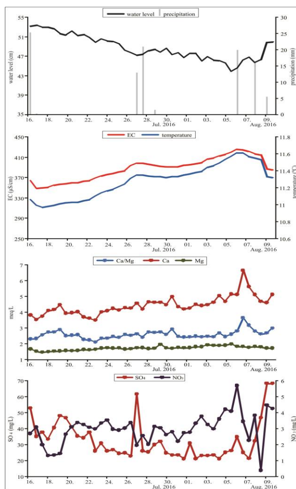
Fig. 7. Variations of water level, electrical conductivity (EC), water temperature and some hydrochemical parameters at the Manastirec spring
