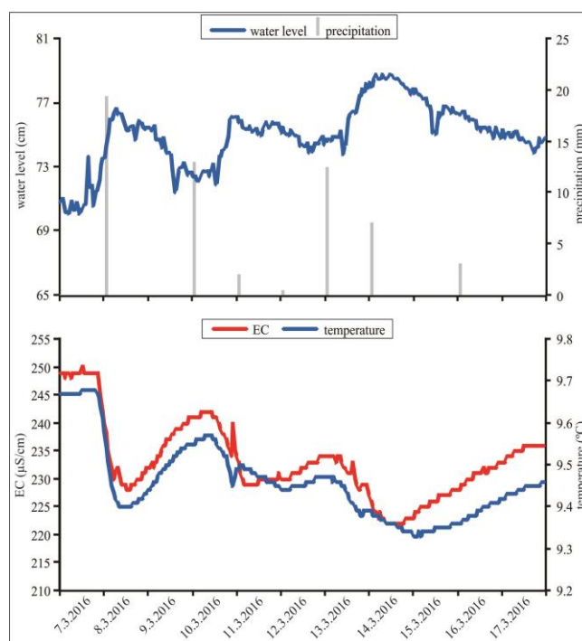
Fig. 5. Measurements of precipitation, water level, temperature and electrical conductivity (EC) in the period between March 7 th and March 17 th 2016, every hour
