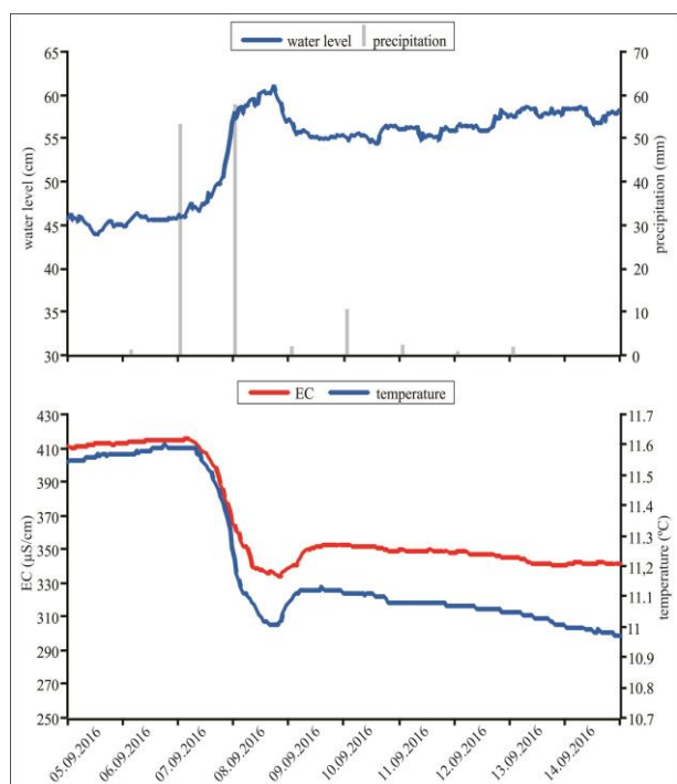
Fig. 6. Measurements of precipitation, water level, temperature and electric conductivity (EC) in the period between September 5 th and September 14 th 2016, every hour
