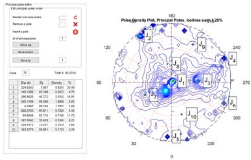
Fig. 2a Pole density plot in DSE from 3DPC. Fig. 2b Identified planes from all methods are marked with similar color.
