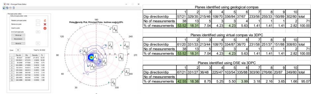
Fig. 1a. Pole density plot in DSE from 3DPC; Fig. 1b. Identified planes from all methods are marked with similar color.
