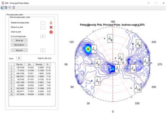
Fig. 3a Pole density plot in DSE from 3DPC. Fig. 3b Identified planes from all methods are marked with similar color.
