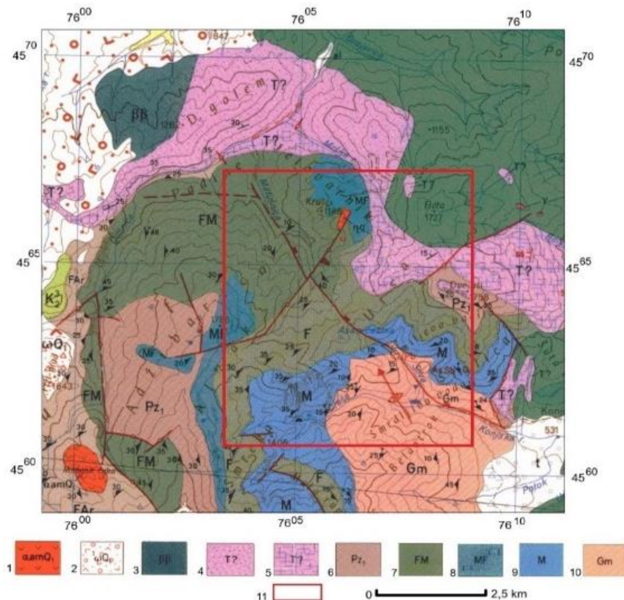
Fig. 1. Geological map of part of the Kožuf area (section of O GK)
