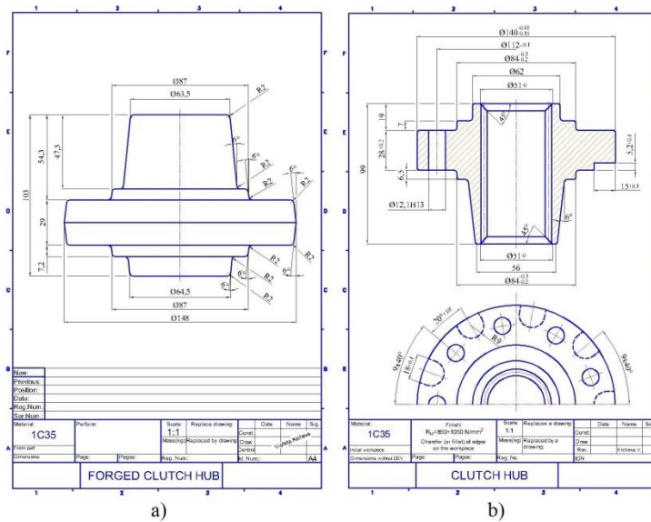
Figure 3. a) Initial forged workpiece; b) Completed clutch hub [8]
