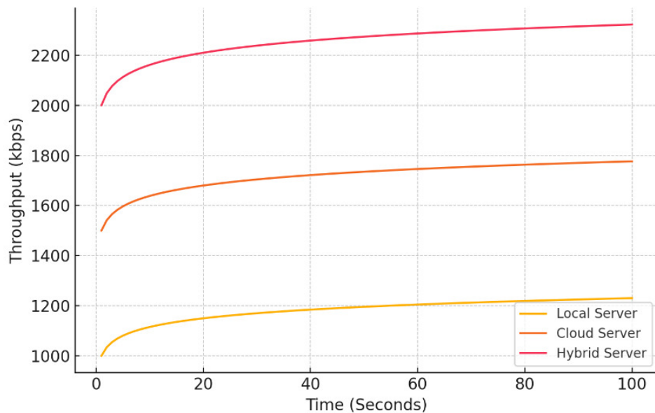
Fig. 6. Message throughput comparison
