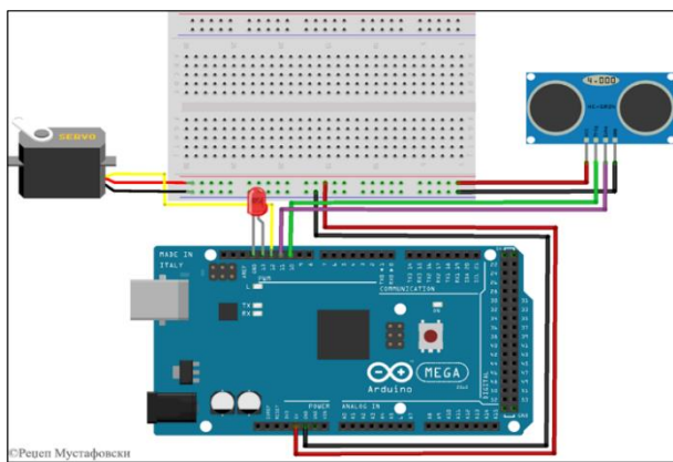
Fig. 6. Connecting the components of the URSAD [15]
