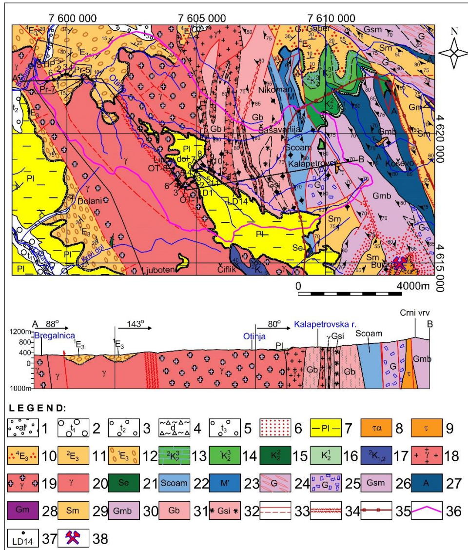
Fig. 2. Geological map of the wider environment of the catchment area of the river of Otinja.
