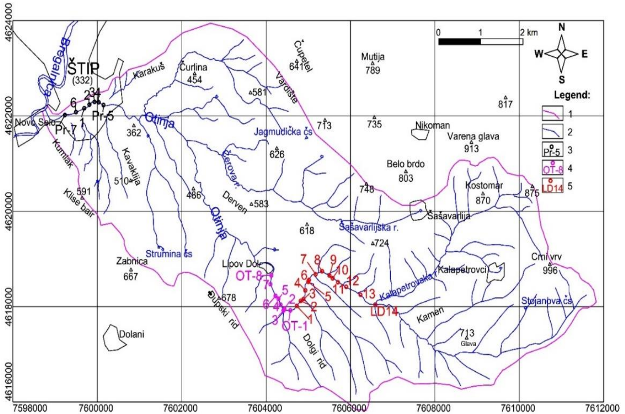
Fig. 3. Schematic map of the catchment area of the Otinja river with the locations of the tested schlich samples. Legend: 1 – Boundary of the catchment area of the Otinja river; 2 – Drainage system; 3–5 – Locations of tested schlich samples on three occasions
