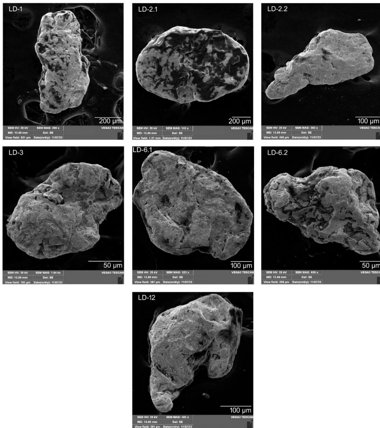
Fig. 6. Scanning electron microscope (SEM) photographs of Au grains from the Otinja river.
