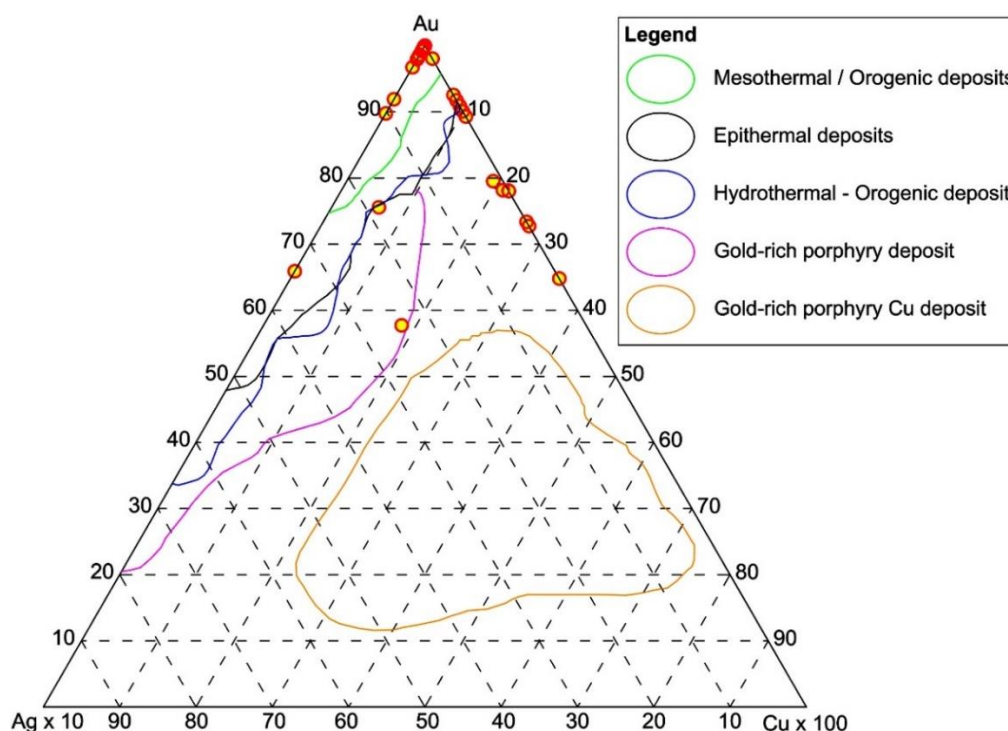
Figure 7. A three-component separation diagram Au–Ag*10 vs. Cu*100 with the composition of Au grains from the Otinja river ( n = 36 )
