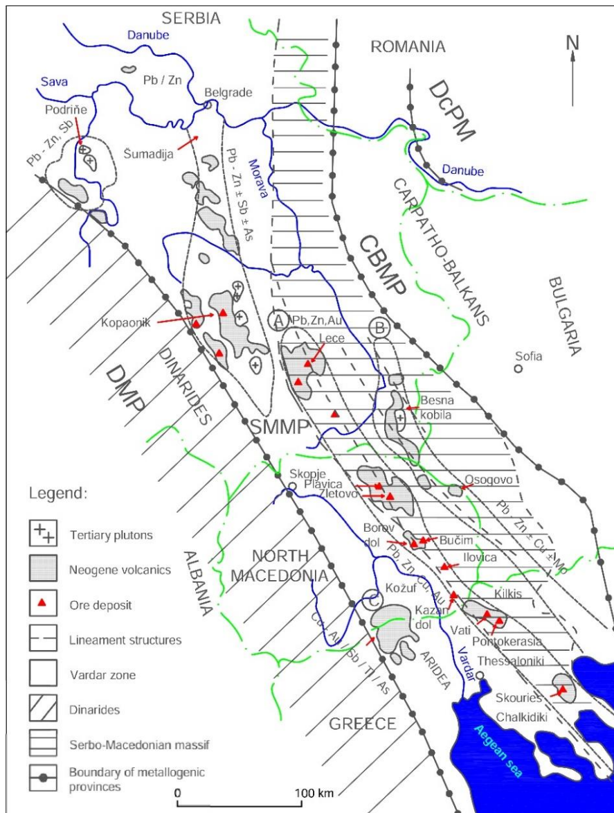
Fig. 1. Main metallogenic zones in the Serbo-Macedonian metallogenic province (modified, according to Janković, 1990).
