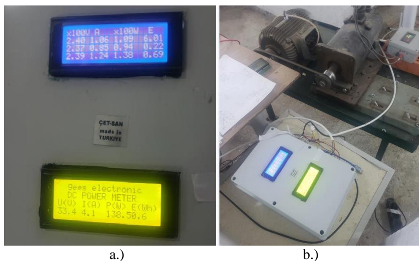
Fig. 12. Realized devices used for testing on AC motor regulator: a.) Integrated AC/DC power meter, and b.) mechanically coupled on the AC motor by a DC generator.
