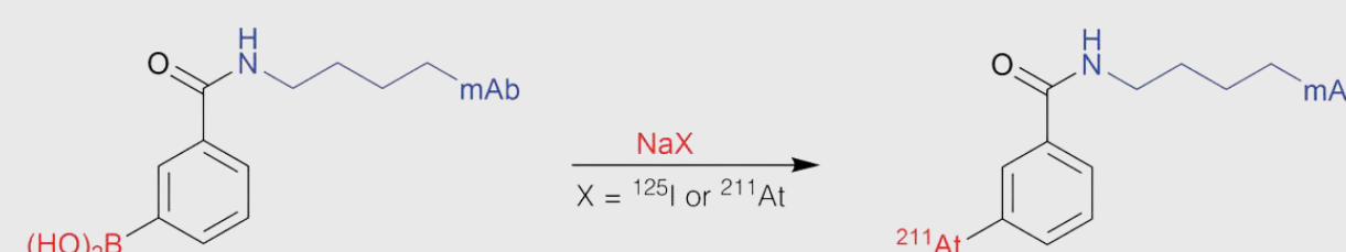
The nucleophilic single-step approach of radiolabeling with astatine-211 or iodine-25
