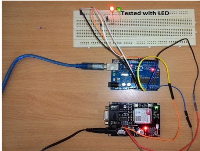
Figure 8. Test version of GSM module in combination with Arduino controller
