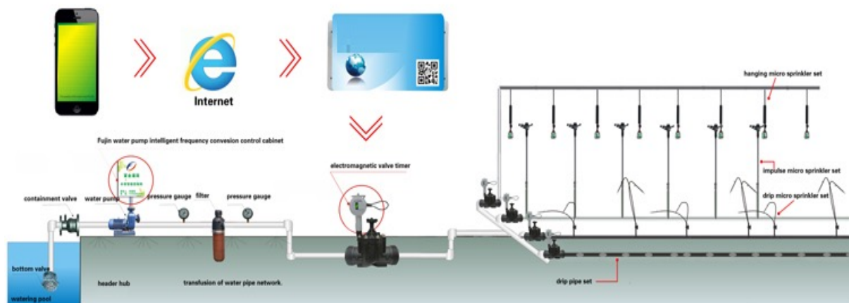
Figure 2. Indication of irrigation by means of pumps operated via a mobile phone
