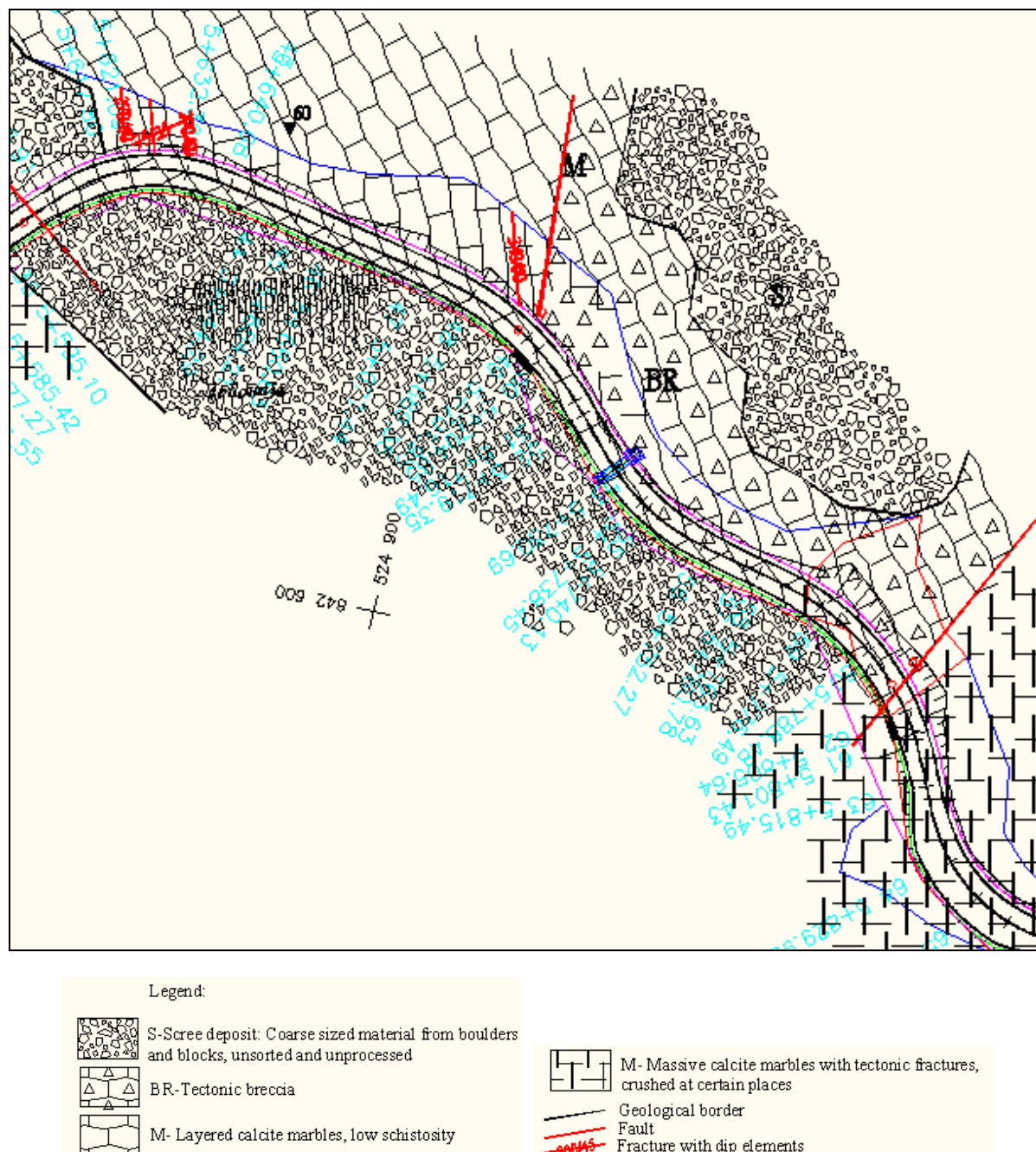
Fig. 1. Engineering geological map for access road to dam Sv. Petka (Chainage km.5+595 – km.6+854)
