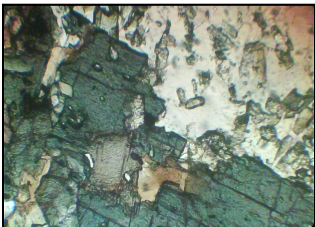
Fig. 6. Microphotography of the amphibolic quartzdiorite of the Kosovska river locality. Parallel nicols, magnified 10×.
