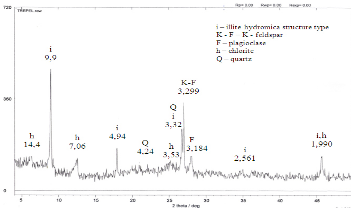
Fig. 11. X-ray diagram of examined trepelChemical examinations
