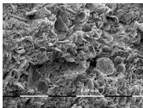
Fig. 9. SEM-photo of a common trepel mass composed of numerous microrelics – opal globules of biogenetic origin
