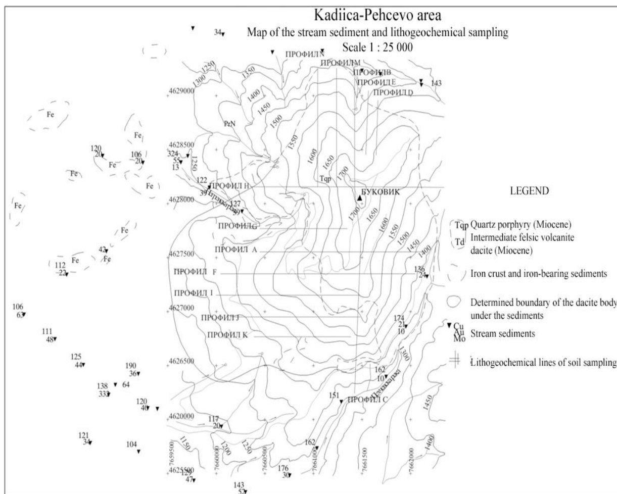
Fig. 4. Map of the lithogeochemical sampling and stream sediments (Aleksandrov and Bombol., 2007)
