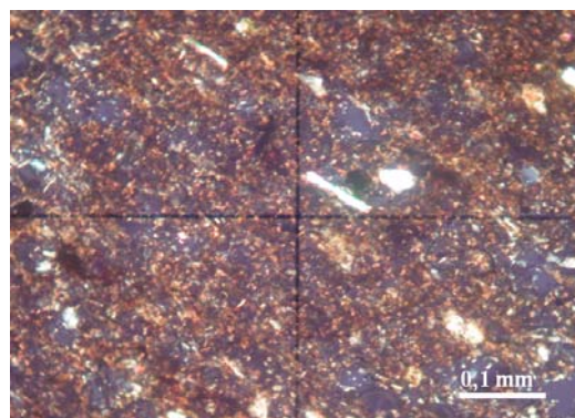
Fig. 4. Superfinegrained quartz, feldspars, illite, chlorite, (like spots and fibres) enclosed in the finegrained opal structure of biogenetic origin (N + )
