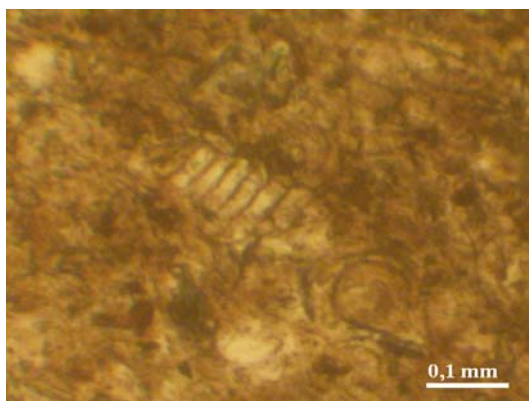
Fig. 7. Non yet determined microfossil of zoogenethic origin in the trepel mass ( N^+ )
