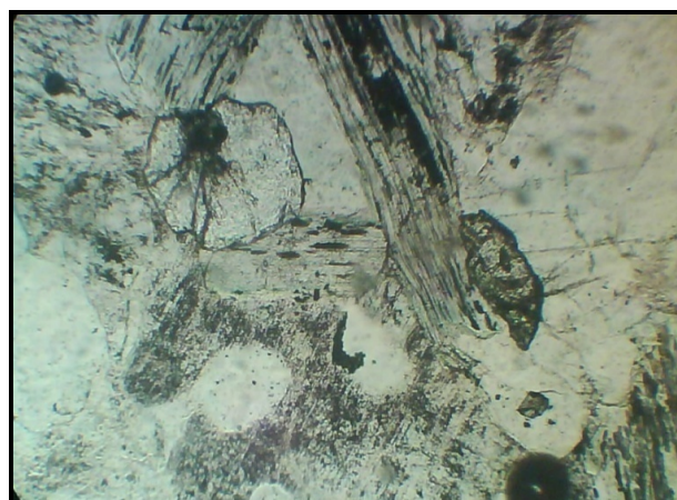
Fig. 10. Microphotography of the thin striped muscovite gneiss of the Kosovska river locality. Parallel nicols, magnified 10×.
