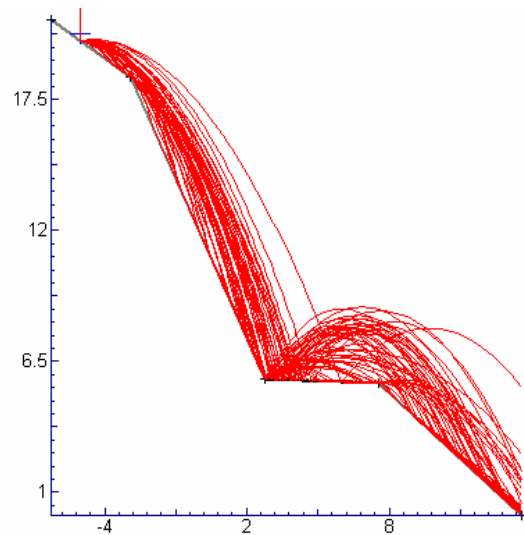
Fig. 3. Output of Rocscience program RocFall from detailed analysis
