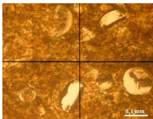
Fig. 5. Isotropic globular structure of trepel composed mainly of opal globules (N + )
