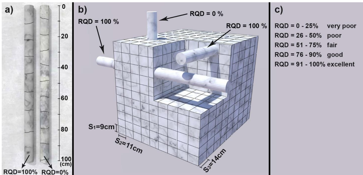
Fig. 2. a) Limitations in the traditional methodology can generate different RQD values even due to a small change in the size of core sticks, b) Sensitivity and dependence of RQD values on drilling direction of the borehole, c) RQD index classification values of rock mass
