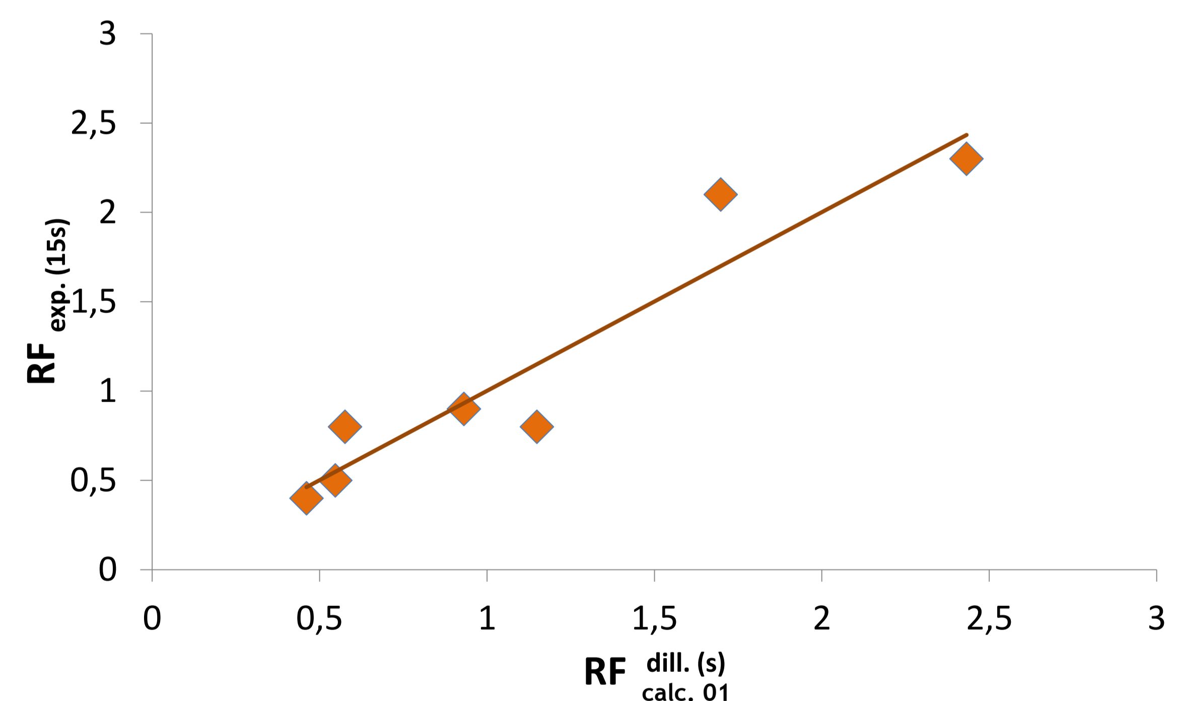
Fig. 1. Plot of the observed disinfection activity to S. aureus , after 15s of exposition (RF exp. (15s) ) vs the calculated activity with DACS 1 (RF calc. 01 dil. (s) )
