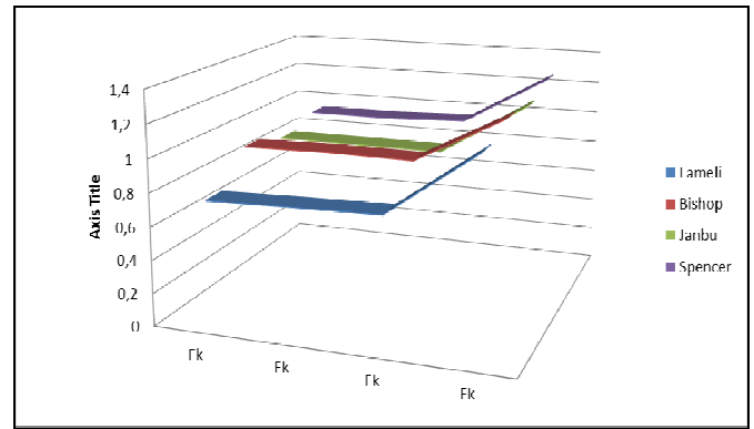
Figure 1 Factor of Safety on Section P08-P08'
