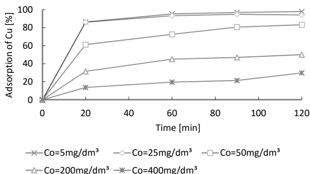
Fig. 4. Effect of initial \text{Cu}^{2+} concentration on the adsorption efficiency onto zeolite (5 g of zeolite, pH 3.5)
