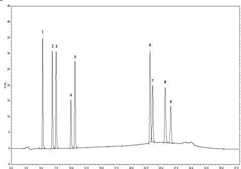
Figure 1. A typical chromatogram of the mixed standard solution containing: dexamethasone (1), prednisolone (2), methylprednisolone (3), fluocortolone (4), hydrocortisone (5), mometasone (6), betamethasone (7), beclomethasone (8), and diflucortolone (9).
