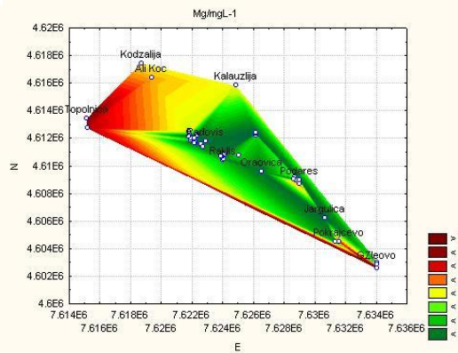
Fig.5. Spatial distribution of Mg 2+ /mgL -1
