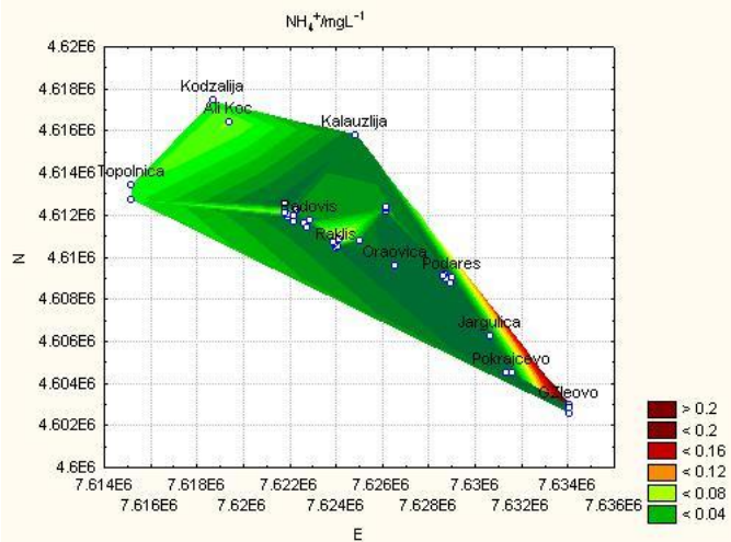
Fig.14. Spatial distribution of \text{NH}_4^+/\text{mgL}^{-1}
