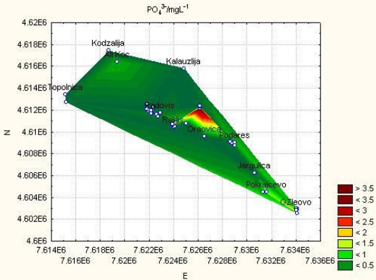
Fig.11. Spatial distribution of \text{PO}_4^{3-}/\text{mgL}^{-1}
