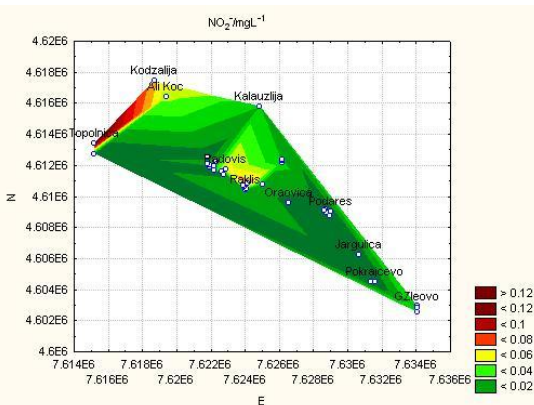
Fig.13. Spatial distribution of \text{NO}_2^-/\text{mgL}^{-1}
