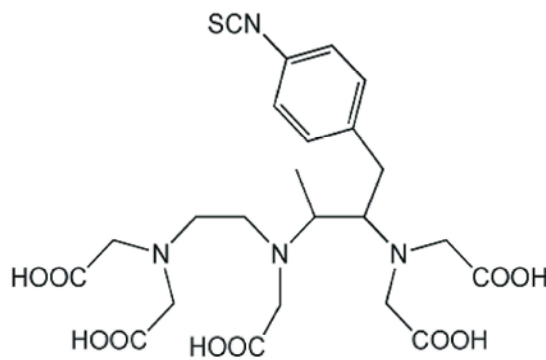
Fig. 3: Structure of used 1B4M-DTPA for rituximab conjugation
