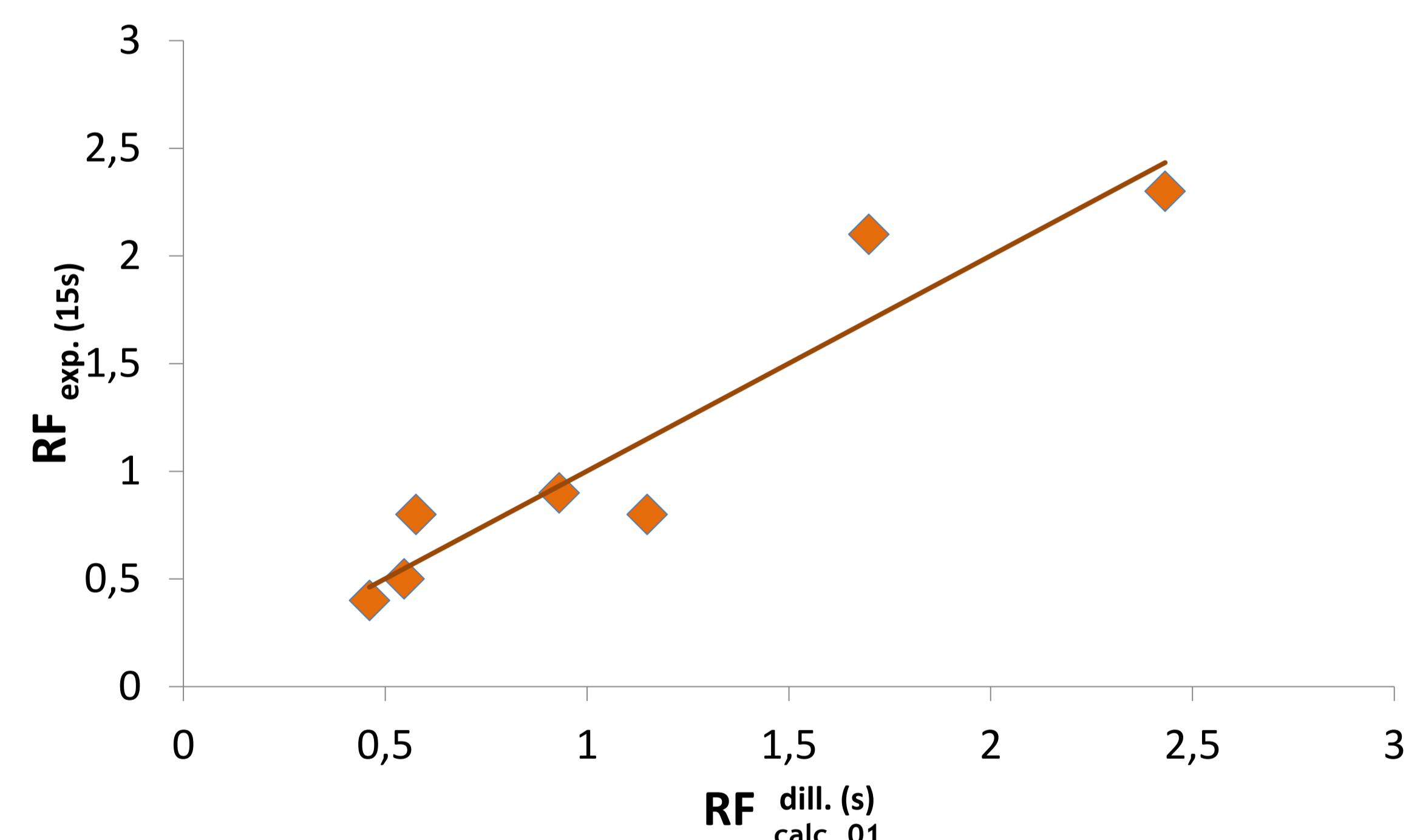
Fig. 1. Plot of the observed disinfection activity to S. aureus , after 15s of exposition (RF exp. (15s) ) vs the calculated activity with DACS 1 (RF dill. (s) )
