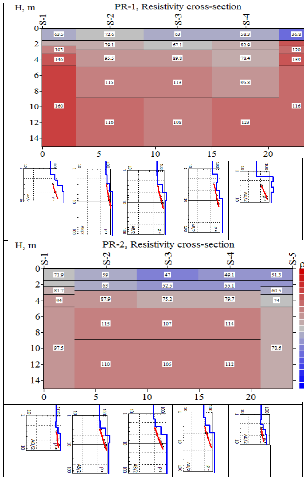
Fig. 3 Models of the specific electrical resistance
