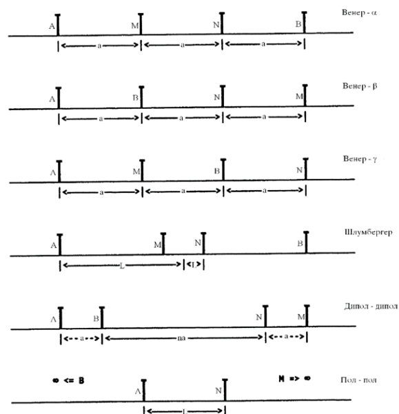
Fig. 1 Examples of different schedules of electrodes (A и B are electrical electrodes, M и N are potential electrodes)
