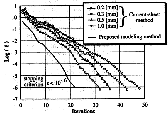
FIG. 3. Convergence rate.
