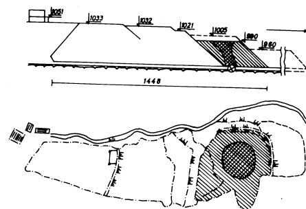
Fig. 1 Cross sections of the Sasa tailing pond.
