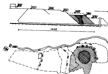
Fig. 1 Cross sections of the Sasa tailing pond.
