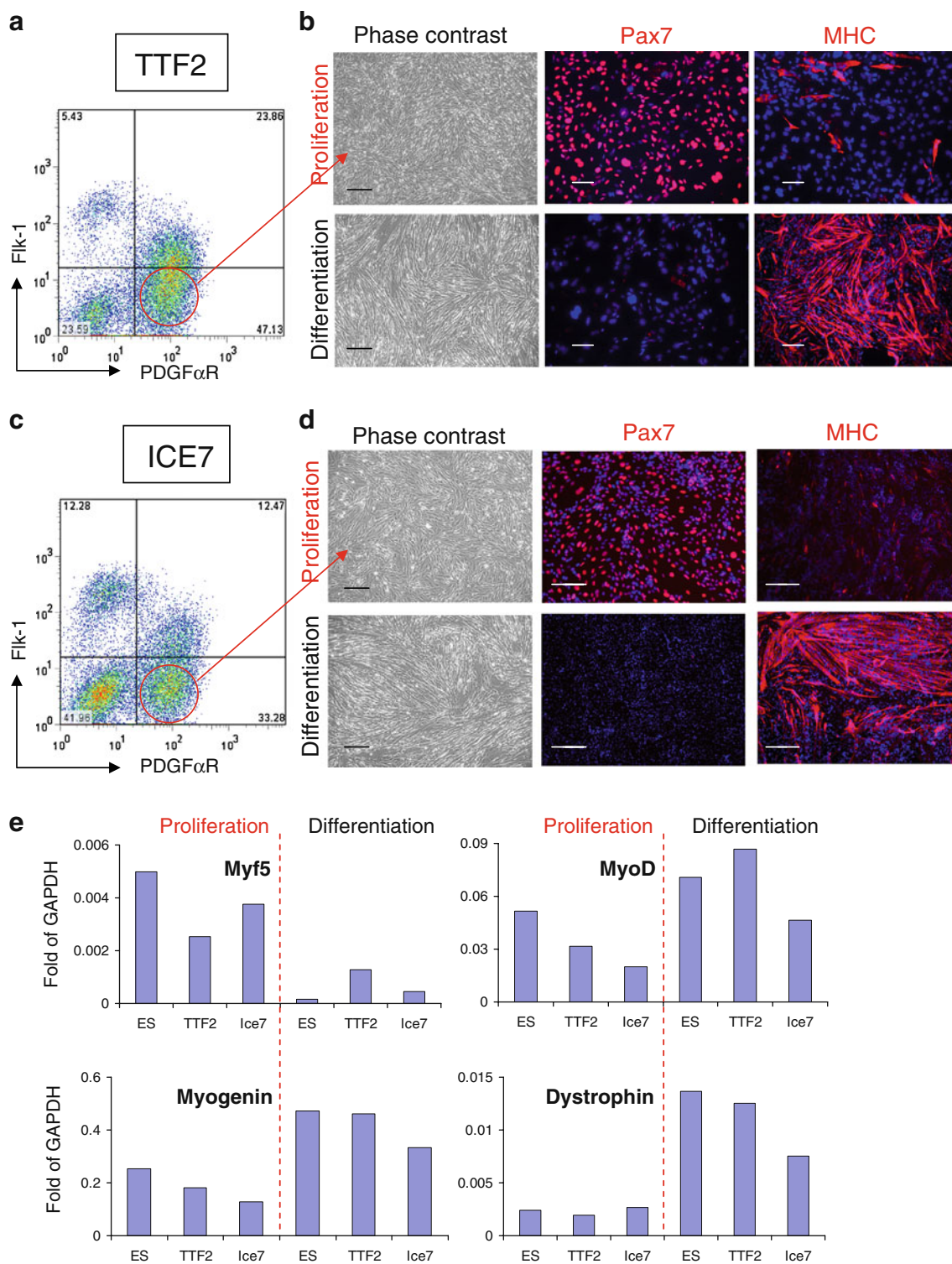
Fig. 3 In vitro myogenic differentiation of iPax7 iPS cells. (a, c) Representative FACS profile of day 5 EBs from TTF2 (a) and ICE7 (c) iPax7 iPS cells for PDGF \alpha R and Flk-1 expression. Dox was added to the EB medium beginning at day 2. Fluorescence intensity for Flk-1 (APC-conjugated) is indicated on the y axis and PDGF \alpha R (PE-conjugated) on the x axis. (b, d) Representative images of TTF2 (b) and ICE7 (d) iPS cell-derived monolayers resulting from the sorting for PDGF \alpha R + Flk-1 - (a, c) under proliferation (upper panel) and
