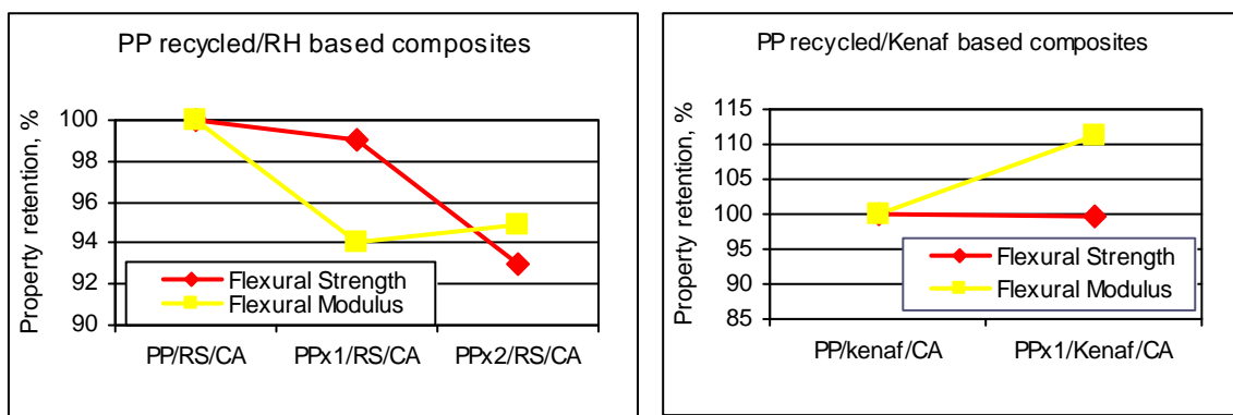
Fig. 1.a) Influence of the recycled PP on the properties of the PP/RH and PP/kenaf composites
