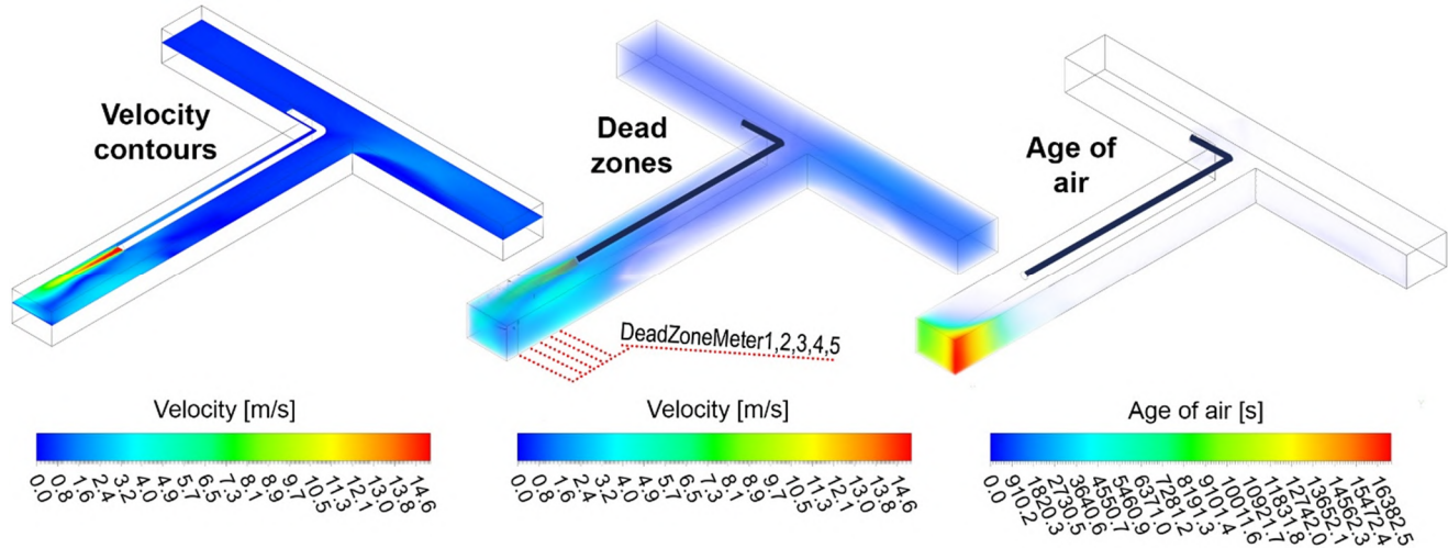
Figure 12. CFD simulation of the calculated optimal distance from the outlet of the auxiliary forcing ventilation system to the development heading (Candidate Point 1).
