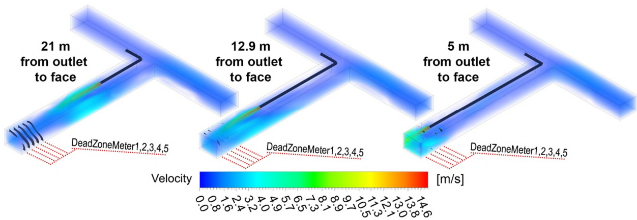
Figure 8. Dead zone areas for different outlet locations.
