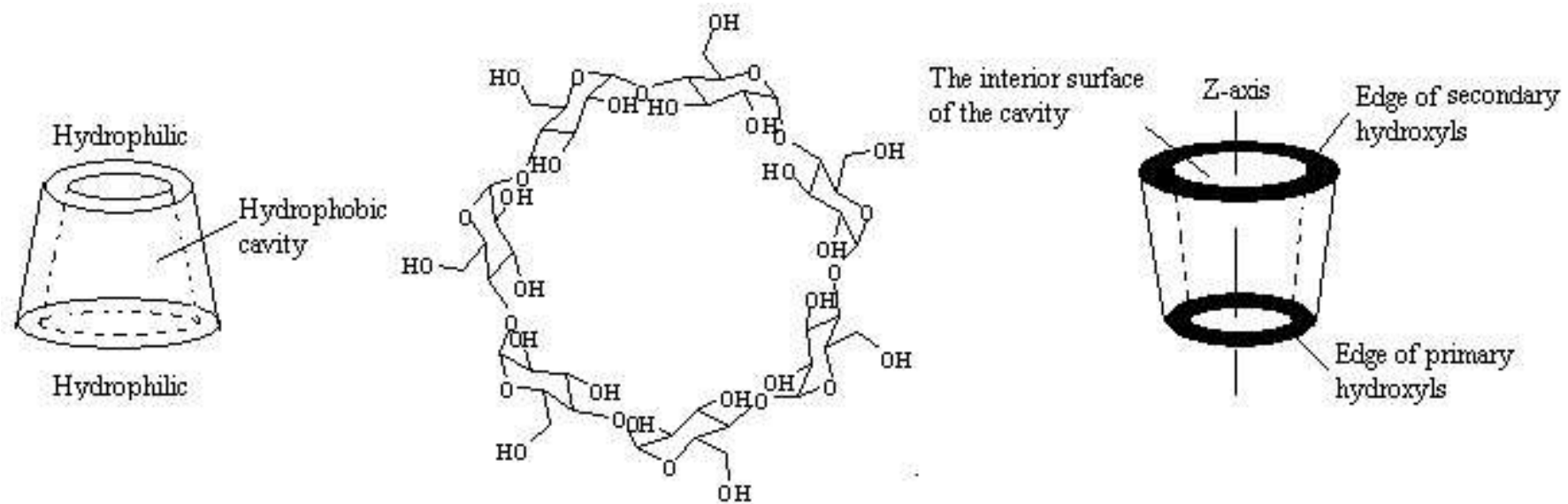
Fig.1. Structure of \beta -cyclodextrin
