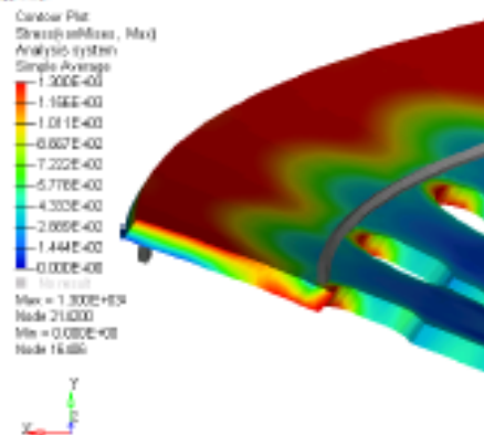
Fig.12 Complex stress at the disengaged position 0392/0313
