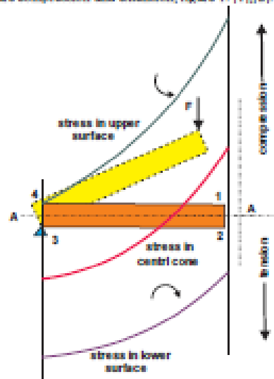
Fig.1 Spring stresses
