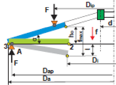
Fig.3 Spring with one supporting point
