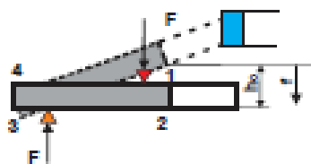
Fig.2 Diaphragm spring with its supporting points
