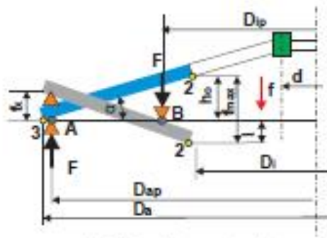
Fig. 4 Spring with two supporting points
