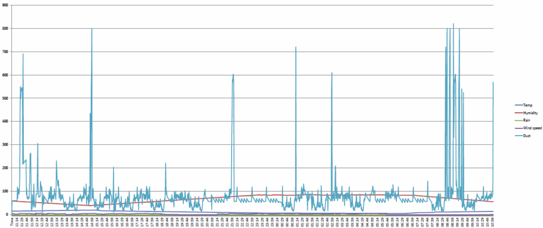
Fig. 2. Daily distribution of PM_{10} particulate matter in the Tikveš area
