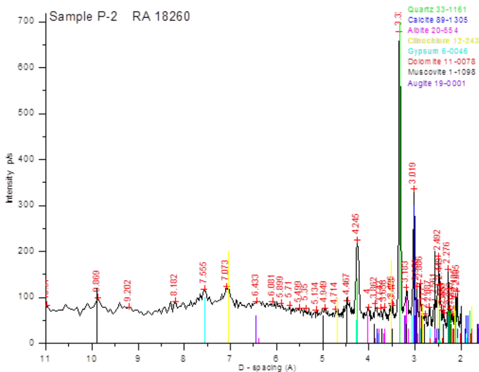
Fig. 3. X-ray diffractogram of \text{PM}_{10} (sample No. 2)
