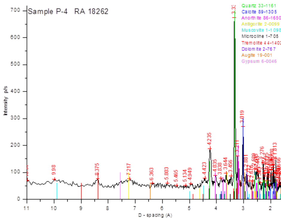
Fig. 4. X-ray diffractogram of \text{PM}_{10} (sample No. 4)
