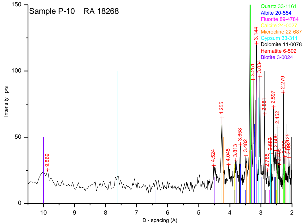
Fig. 6. X-ray diffractogram of PM_{10} (sample No. 10)
