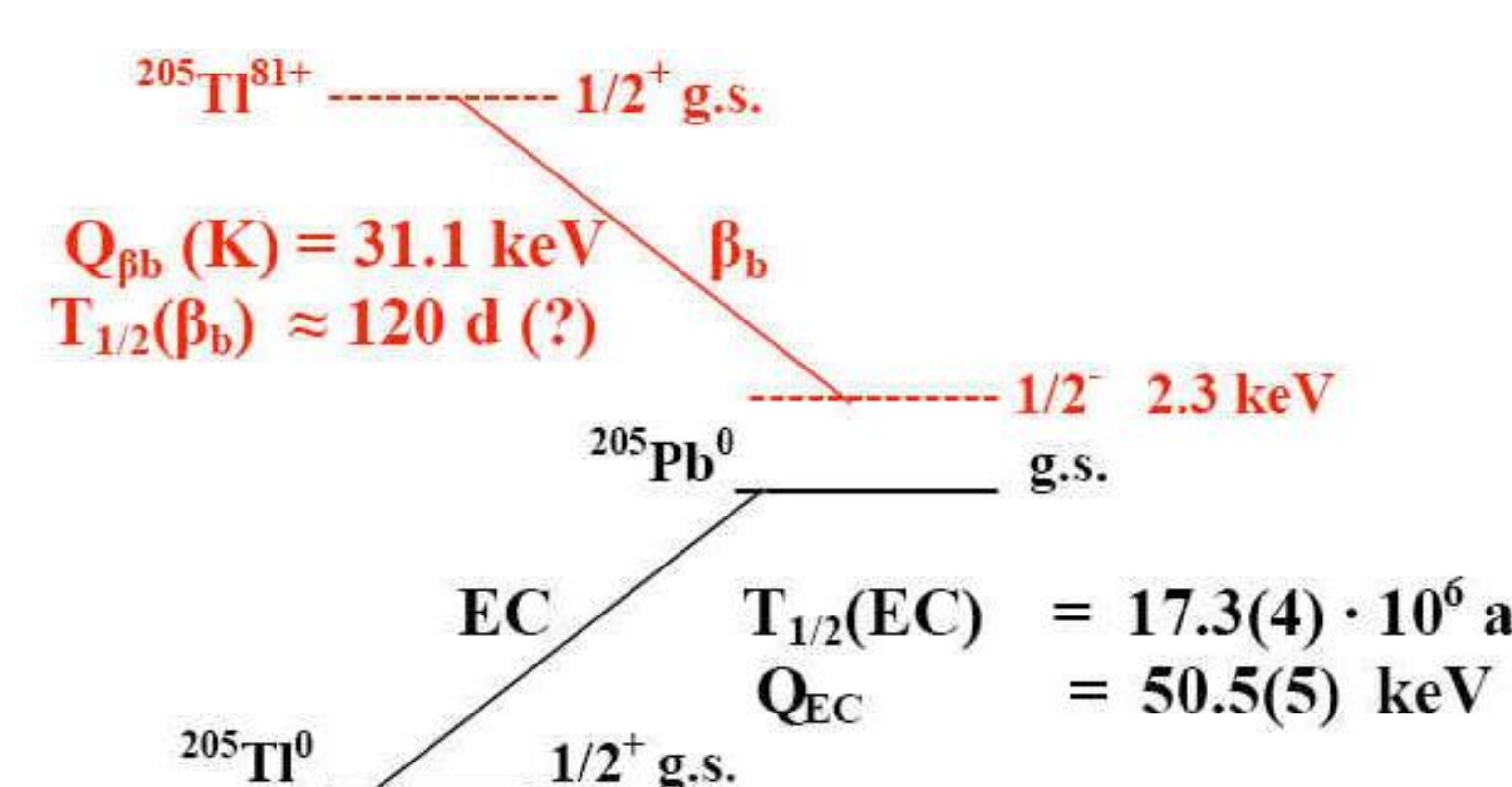
Fig.2. Decay scheme of neutral ^{205}\text{Pb} atoms (black) and of bare ^{205}\text{Tl}^{81+} ions (red). Whereas neutral ^{205}\text{Pb} atoms decay by unique first-forbidden orbital electron capture (EC) from the L and higher electron shells to stable neutral ^{205}\text{Tl} atoms with a half-life of 17.3 million years and a Q value of 50.5 keV, bare ^{205}\text{Tl}^{81+} (or H-like ^{205}\text{Tl}^{80+} ) ions can decay to almost 100% by \beta_b decay to the first excited state of ^{205}\text{Pb} - ^{205}\text{Pb}^{81+} at E^* = 2.3 \text{ keV} , where the generated electron will be captured into the K shell (5).
