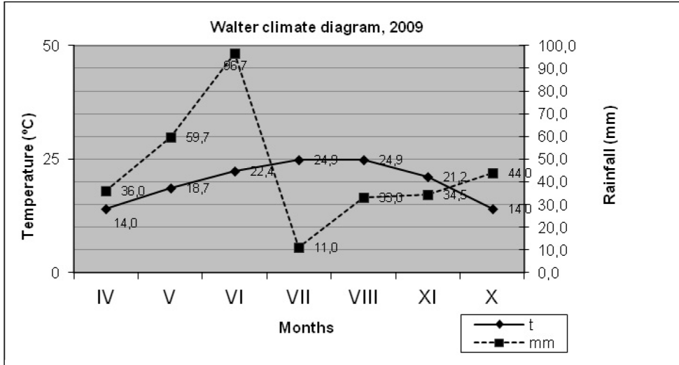
Figure 1. Walter climate diagram for 2009
