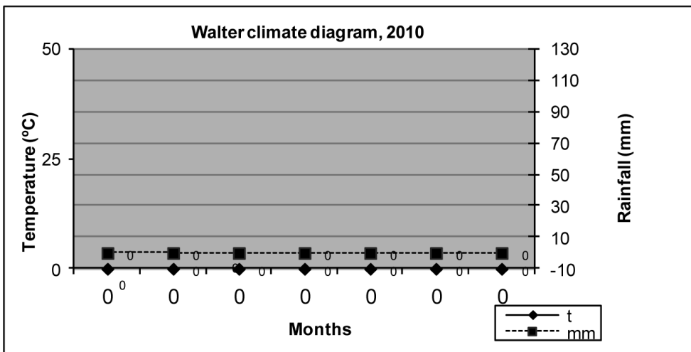
Figure 2. Walter climate diagram for 2010
