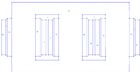
Fig. 2. CAD drawing of three phase transformer
