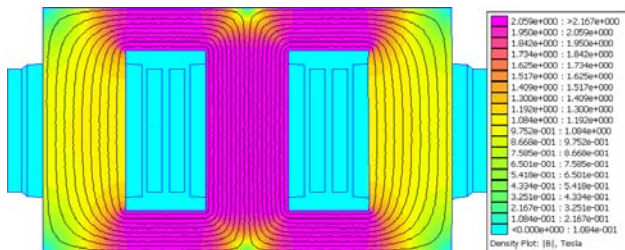
Fig. 17. Magnetic flux distribution in transformer-no load.
